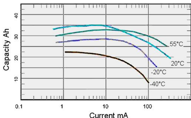
Temperature characteristics
